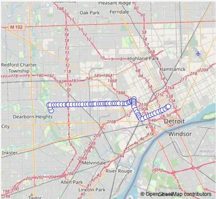
47 — Tireman BusMaps
